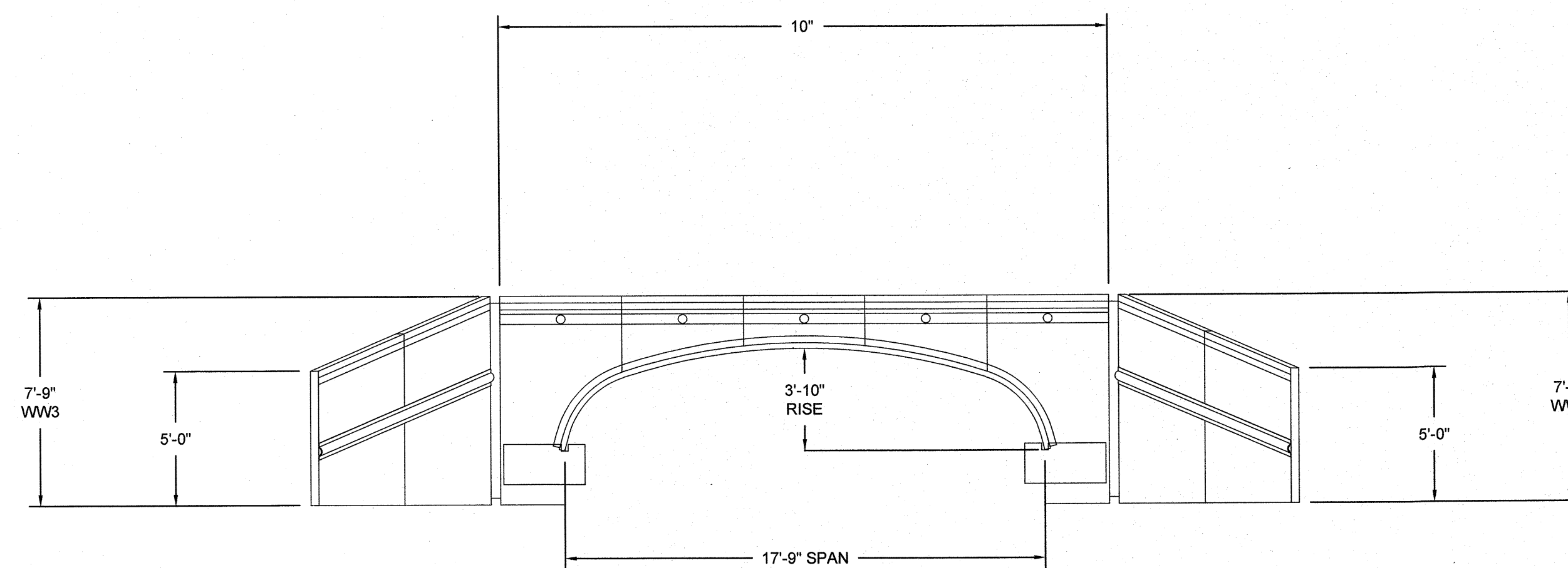
OUTLET END ELEVATION NOT TO SCALE
